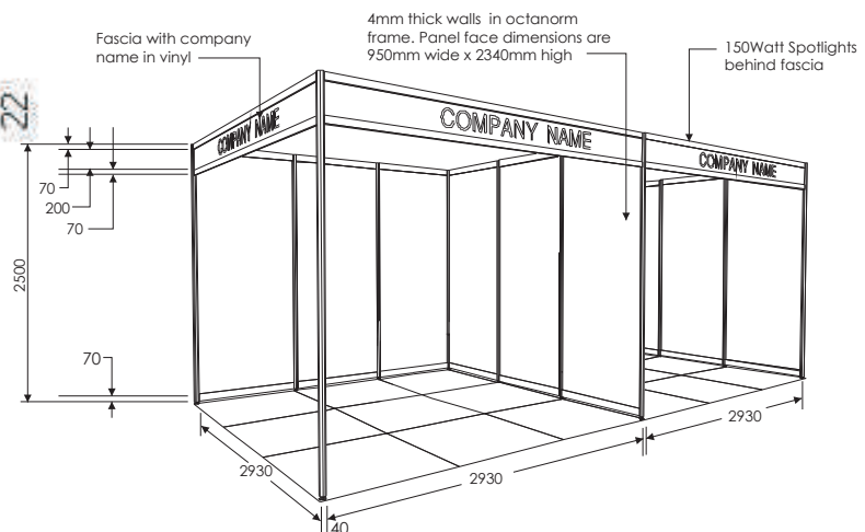
• Overall Booth Drawing (3m x 3m)
