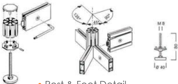
• Post & Foot Detail
