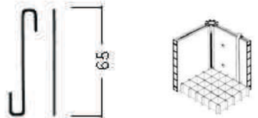
• Optional S-Hook With Hanging Detail Off Top Beam
